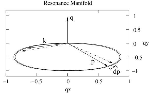
Figure 1: The manifold of wave-numbers that interact resonantly with a p_x = 0 mode. In a full spectrum one should integrate over the other two wave-numbers of the triad to compute the diffusion coefficients [as in Eqns. (4-6)], only taking the resonant interactions into account. This can be achieved by computing the integrals along the resonance manifold as shown (up to a wave-number dependent coefficient).
