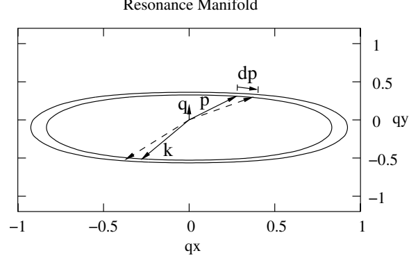
Figure 3: The resonance manifold for the interaction involving a hydrodynamic streamer [i.e. (k_x, k_{\parallel}) \rightarrow 0 ]
