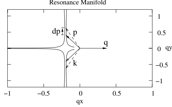
Figure 2: The resonance manifold for the interaction involving a q_y = 0 mode
