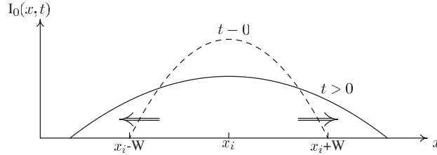
Figure 3. Equation (5) describes a propagating localized front-like solution.
