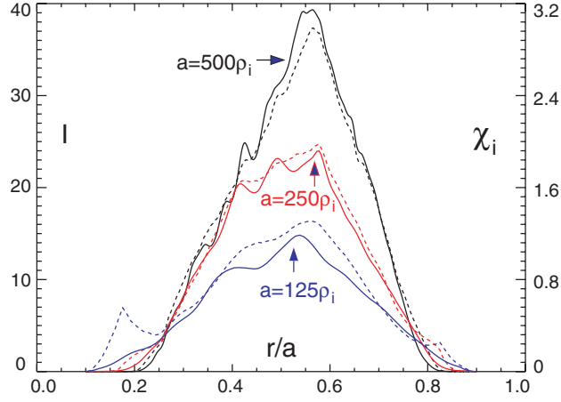
Figure 5. Fluctuation intensity profiles ( I in —) and ion thermal diffusivity ( \chi_i in ····), both in gyroBohm units after nonlinear saturation for a/\rho_i = 125, 250 and 500 : as the system size gets larger, the extent of radial spreading of turbulence into the linearly stable zone gets narrower relative to the system size. It scales with the ion gyroradius \sim 25\rho_i [31].
