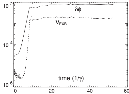
Figure 2. The volume-integrated fluctuation intensity ( \delta\phi ) saturates in magnitude as the self-generated zonal flow ( V_{E \times B} ) grows to a saturated amplitude. The radial spreading of turbulence occurs from approximately t = 8/\gamma , while the volume-integrated fluctuation intensity stays approximately a constant in time.
