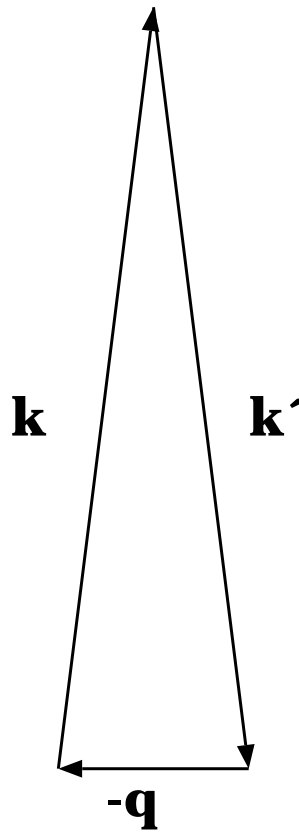
Fig. 3.— Three-wave interaction of two nearly opposite Alfvén quanta \mathbf{k} and \mathbf{k}' with a long wave acoustic wave \mathbf{q} .
