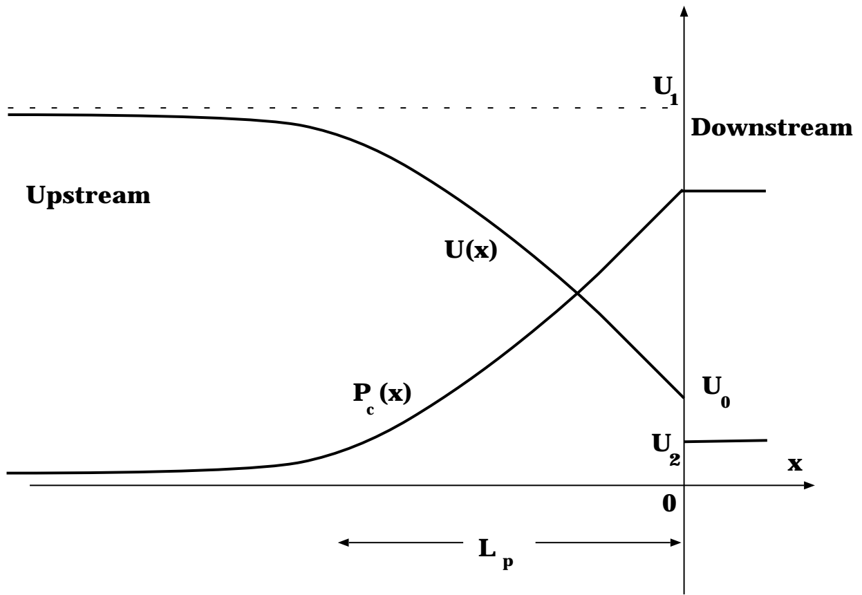
Fig. 2.— The structure of a CR modified shock, with the flow profile U(x) and CR pressure distribution P_c(x) . The sub-shock is at x = 0 and the CR precursor of the length L_p is formed upstream, x < 0 .
