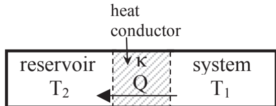
FIG. 3: The system (superconductor in a magnetic field) at initial temperature T_1 is connected to a heat reservoir at temperature T_2 < T_1 through a heat conductor of thermal conductivity \kappa . The entire assembly is thermally and mechanically insulated from its environment.
