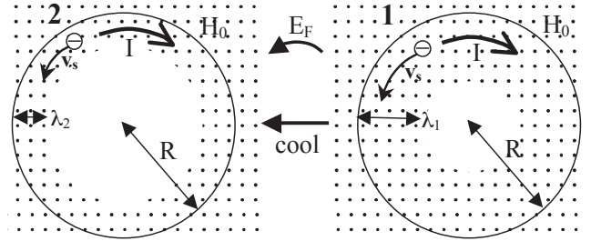
FIG. 2: Cylindrical superconductor seen from the top. The right (left) panel indicates the system in the state 1 (2) of Fig. 1. The dots indicate magnetic field H_0 coming out of the paper. The same current I flows in both states. The Faraday electric field E_F generated during the process points counterclockwise.
