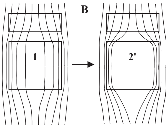
FIG. 8: Same superconducting cylinder as in Fig. 7, with a normal metal cylinder added on top (smaller rectangle) The figure shows schematically the situation where the normal metal is a perfect conductor, or equivalently the transition occurs infinitely fast, so the field lines are frozen in the normal metal.
