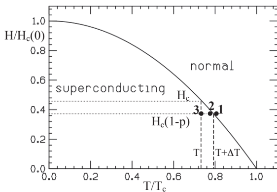
FIG. 4: In the figure, state 1 corresponds to the normal state at the coexistence line and state 2 to the superconducting state at the coexistence line. State 3 is a state at a slightly lower temperature.
